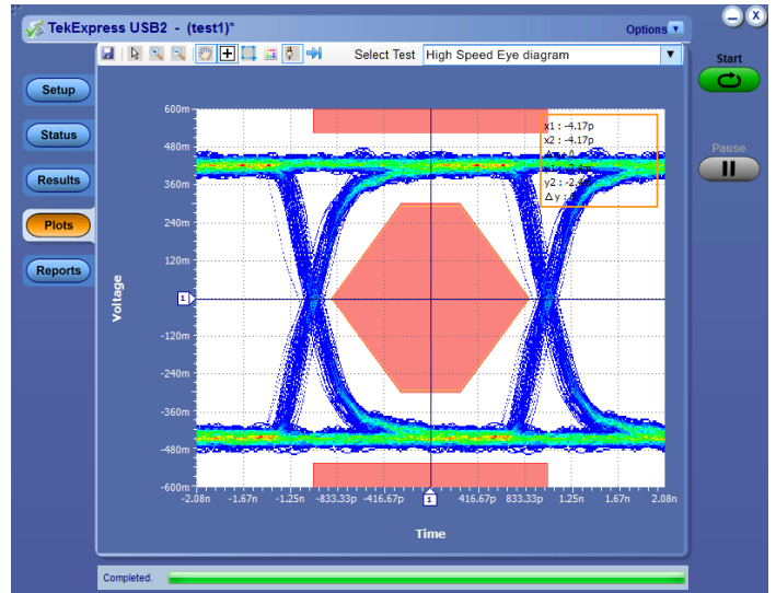
USB 2.0 Automated Compliance Testing.
